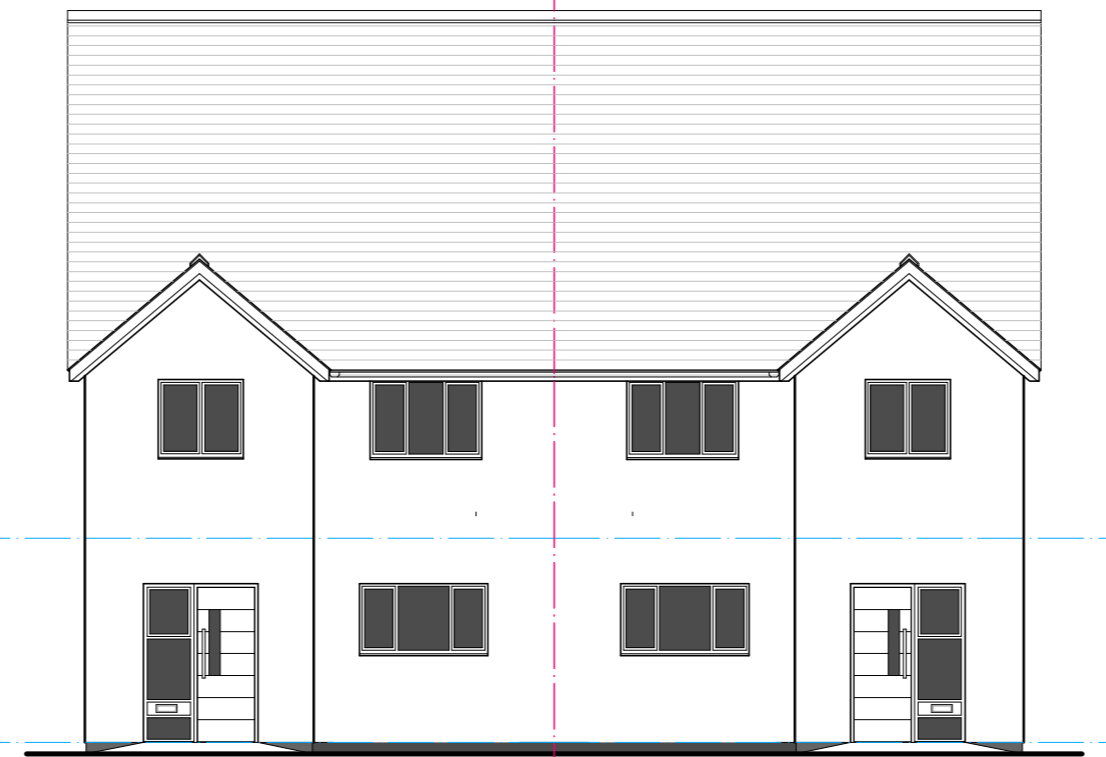
NORTH EAST (ROAD) ELEVATION
